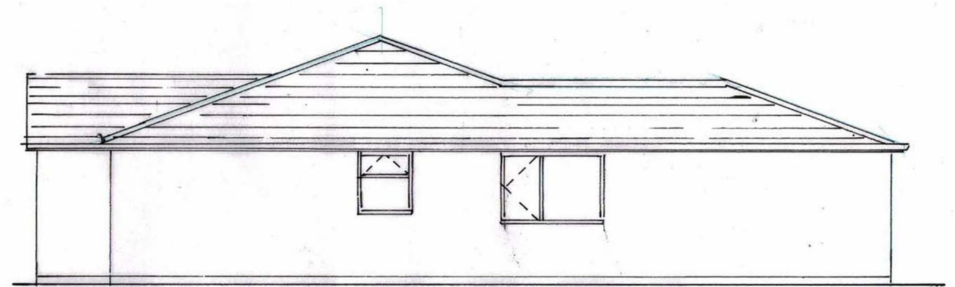
SIDE ELEVATION N.West
